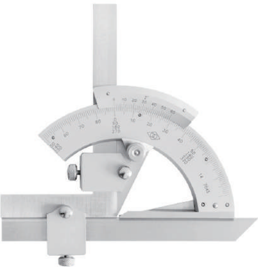
UNIVERSAL BEVEL PROTRACTORS 613
